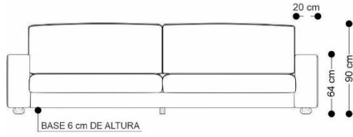
VISTA FRONTAL
